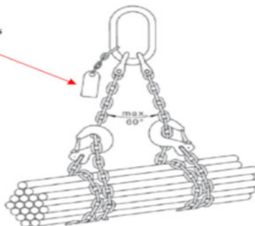
Identifiable markings on Chain Slings
